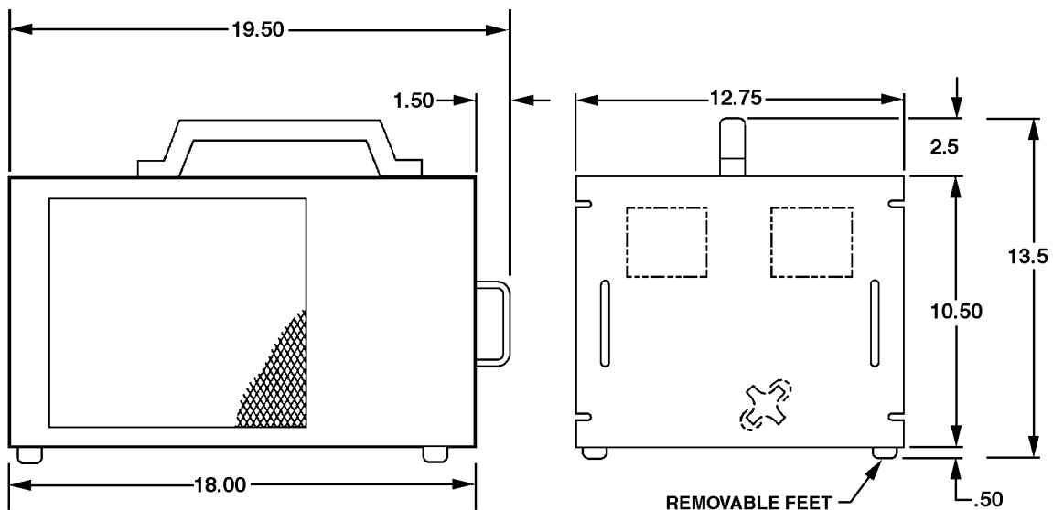
EXHAUST SIDE
